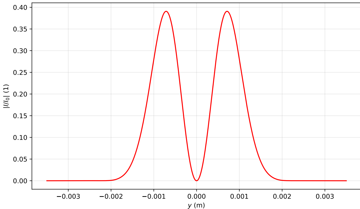
Intensity profile I(x=0, y, z=2.149)/I_0 , P_{in}=1.0P_{cr} , artificial time
